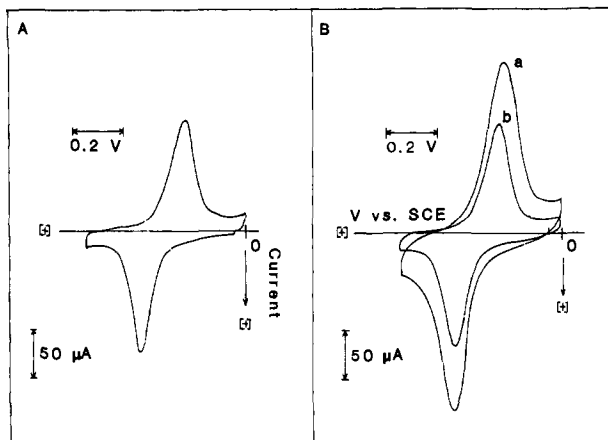
Figure 14. CV on two Pt/mica electrodes each covered with ca. 300 Å of PVFAN in an aqueous 0.5 M NaClO_4 solution at a scan rate of 100 mV/s. (A) One electrode connected and the other at open-circuit condition and two electrodes are ca. 2 mm apart. (B-a) Repeat experiment A with two electrodes brought together with the two Pt films ca. 1600 Å apart. (B-b) Repeat experiment A after experiment B-a.
