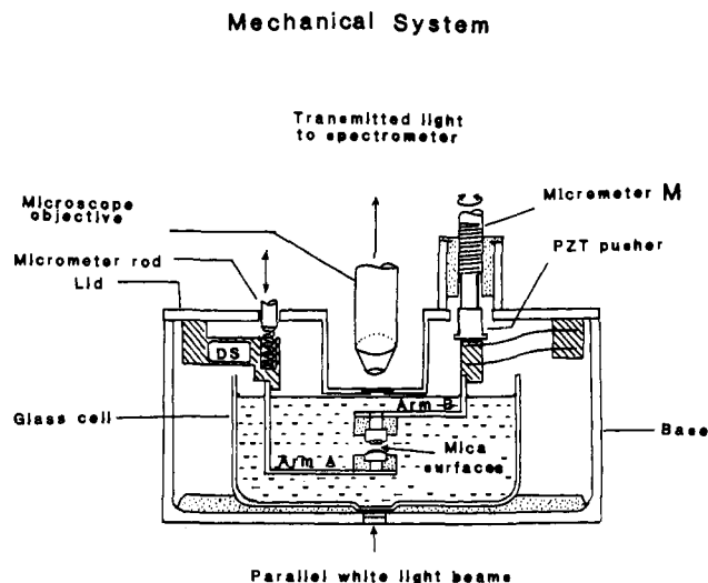
Figure 1. Apparatus for distance adjustment between crossed Pt/mica electrodes. The relative vertical position of the rigid arms A and B, on which cylindrical quartz lenses for Pt/mica sheets are mounted, is controlled via a three-stage mechanism. Coarse adjustment is carried out through micrometer M, on which a piezoelectric (PZT) pusher is attached, with a range of 2–3 mm. A finer adjustment is provided by the differential spring assembly, DS, in which a micrometer-driven rod R pushes a helical spring which in turn acts on a very stiff double-cantilever spring. The ratio of the spring constants of these two springs is ca. 250:1, so that a 1 \mu\text{m} vertical motion of R results in a 40 \text{\AA} vertical displacement of arm A. The final-stage fine control is through the PZT pusher (Model PZ-30, Burleigh Instruments, Inc., Fishers, NY), which moves arm B vertically up or down, depending upon the voltage applied to the PZT element.
