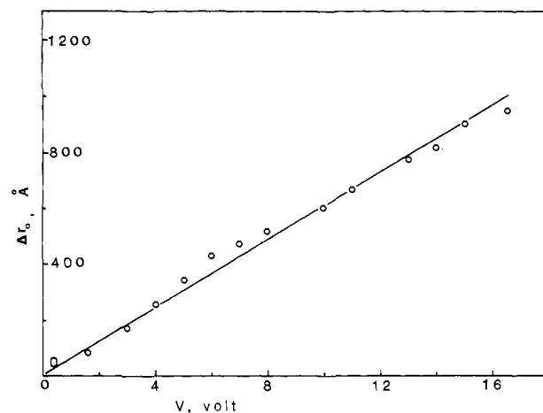
Figure 3. Calibration curve for the displacement of PZT pusher as a function of the applied voltage.
