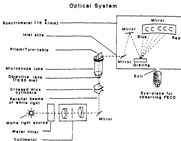
Figure 2. The optical arrangement for white-light multiple-beam interferometry.
